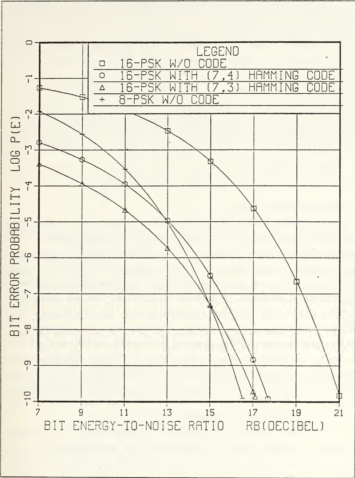
Figure 4.1 Bit error rate comparisons of 16-PSK with and without Hamming code
