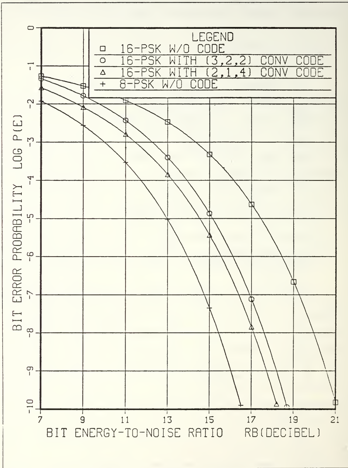
Figure 4.6 Bit error rates of 16-PSK with and without convolutional codes Q = 2
