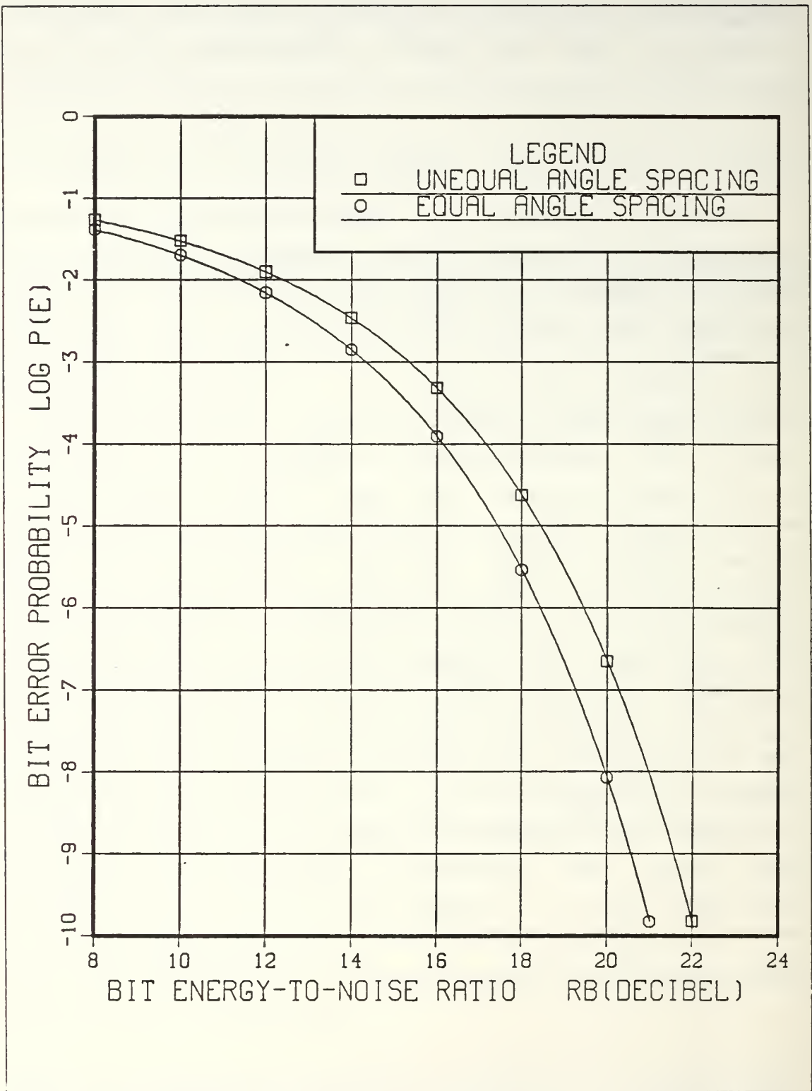
Figure 3.6 Performance of 16-PSK bit detection receiver with equal and unequal angle spacing
