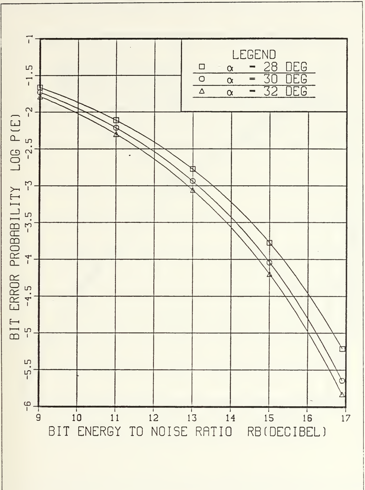
Figure 3.2 (a) Bit error probabilities for 8-PSK with bit detection receiver \alpha = 28^\circ - 32^\circ
