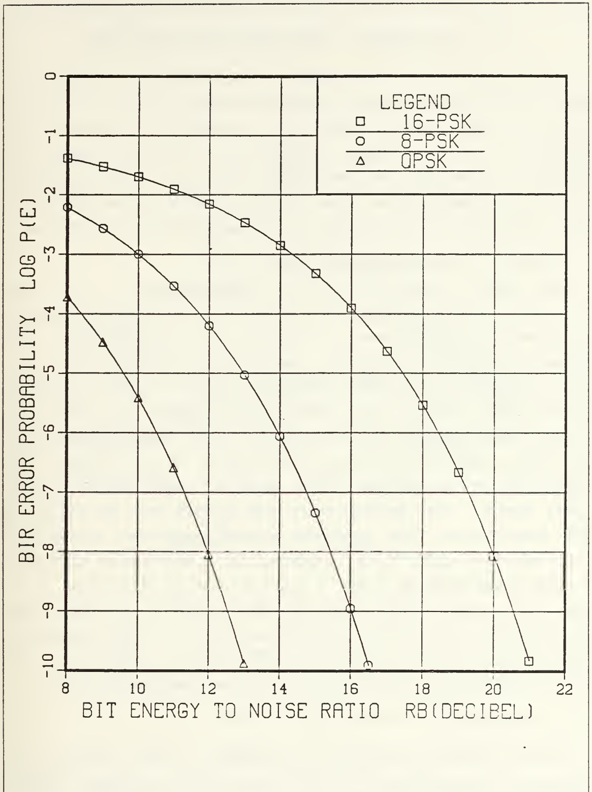
Figure 2.8 Bit error probabilities vs E_b/N_o for 16-PSK, 8-PSK and QPSK
